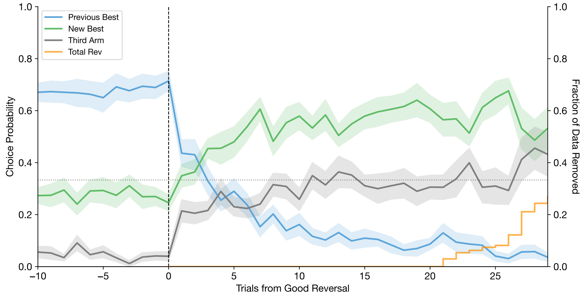
Reversal-Aligned Choices (mean \pm se across problems | n=6 subjects, n=108 reversals, n=14 problems)
